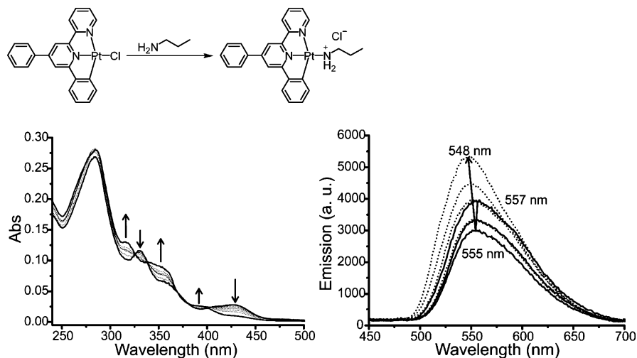
Figure 2. The time-dependent UV/vis and emission spectra of Pt(L)Cl and n -propylamine (1:32).
